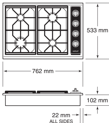
762 mm COOKTOP
