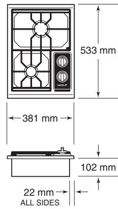
GAS COOKTOP
