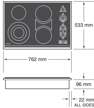
762 mm FRAMED
