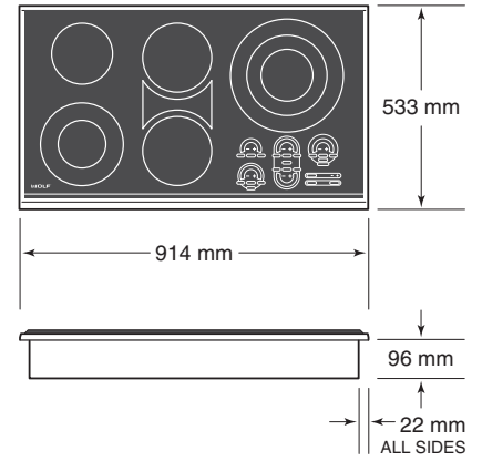
914 mm FRAMED
