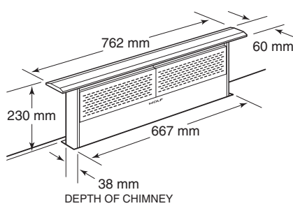
762 mm DOWNDRAFT
