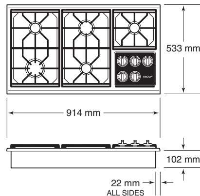
914 mm COOKTOP
