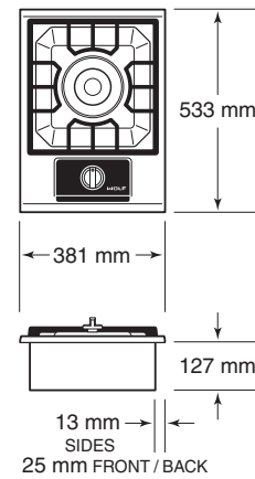
MULTI-FUNCTION COOKTOP
