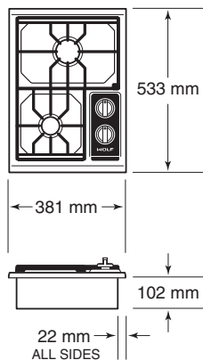
381 mm COOKTOP
