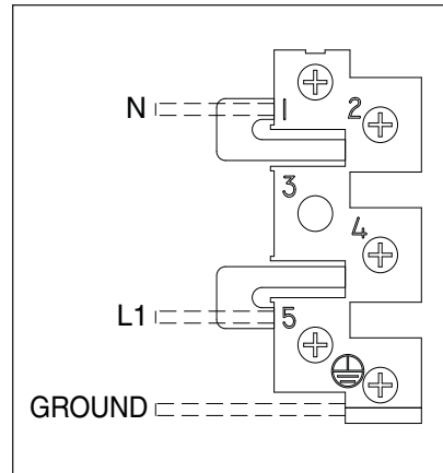
Wiring diagram
